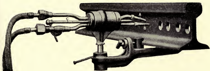
PLATE 23.—Oxy-acetylene blow-pipe for piercing holes in metal rails.
